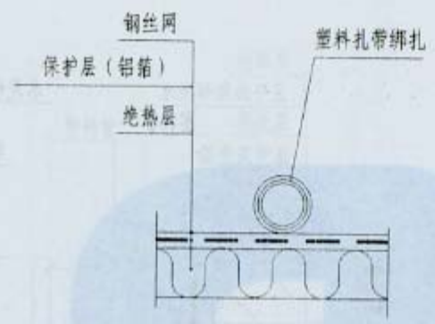
塑料扎带绑扎
